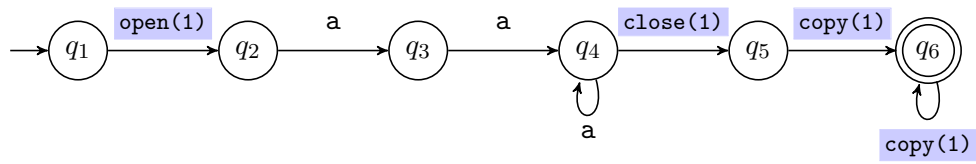
Figure 1: NFA equivalent to the regular expression (aaa^*)\backslash g\langle 1 \rangle \backslash g\langle 1 \rangle^* . Useless epsilon transitions are omitted for simplicity.
